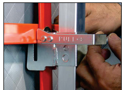
X4702-RUB Roll-up sign bracket
