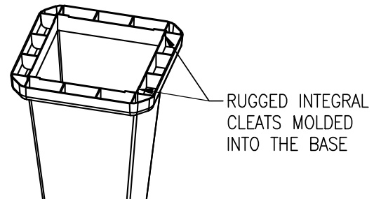
BOTTOM ISOMETRIC
